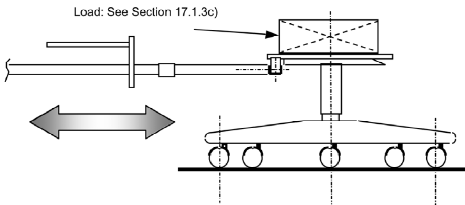
Figure 17c - Machine Schematic for Pedestal Base Chairs
